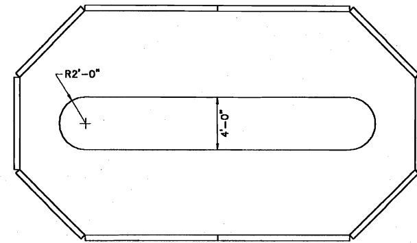
FLAT BOTTOM VOLUME: 8053 IMP GAL
