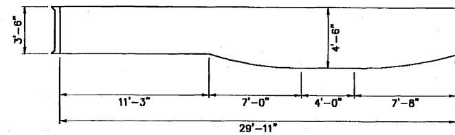
PARTIAL 5' EXPANDABLE BOTTOM VOLUME: 8985 IMP GAL
