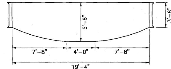
5' EXPANDABLE BOTTOM VOLUME: 7067 IMP GAL
