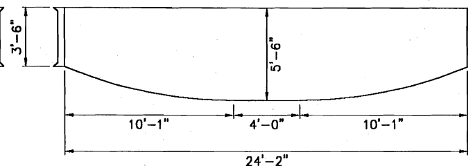
5' EXPANDABLE BOTTOM
