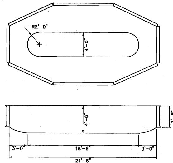
FULL 5' EXPANDABLE BOTTOM VOLUME: 5552 IMP GAL
