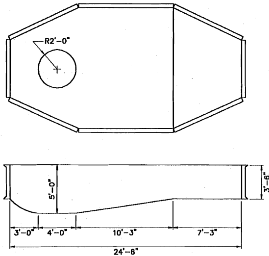
PARTIAL 5' EXPANDABLE BOTTOM VOLUME: 5393 IMP GAL
