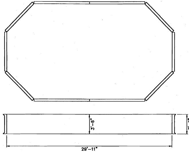
FLAT BOTTOM VOLUME: 8053 IMP GAL
