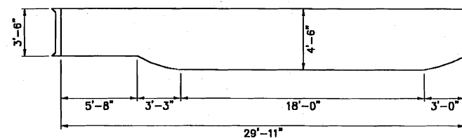
FULL 5' EXPANDABLE BOTTOM VOLUME: 10782 IMP GAL
