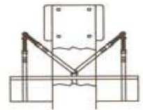
Industry Standard Y-Strap for Under Diving Board
