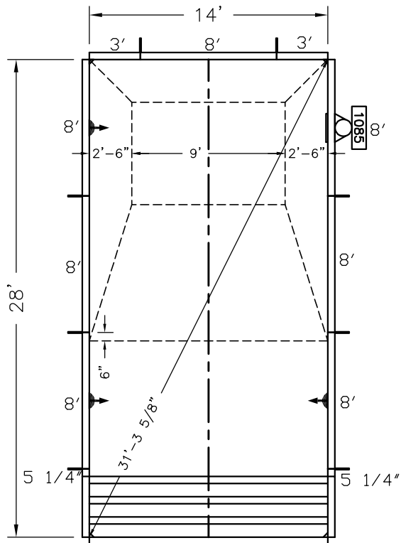
14' POURED STEP W/LINER TRACK SCREED EDGE S1400SP34200XX2
