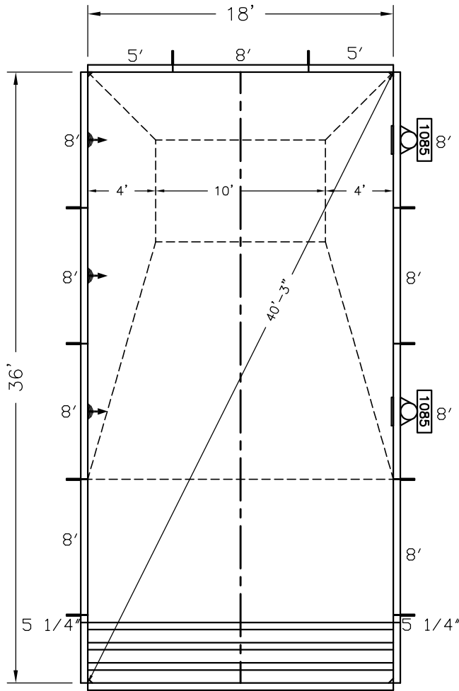
18' POURED STEP W/LINER TRACK SCREED EDGE S1800SP34200XX6
