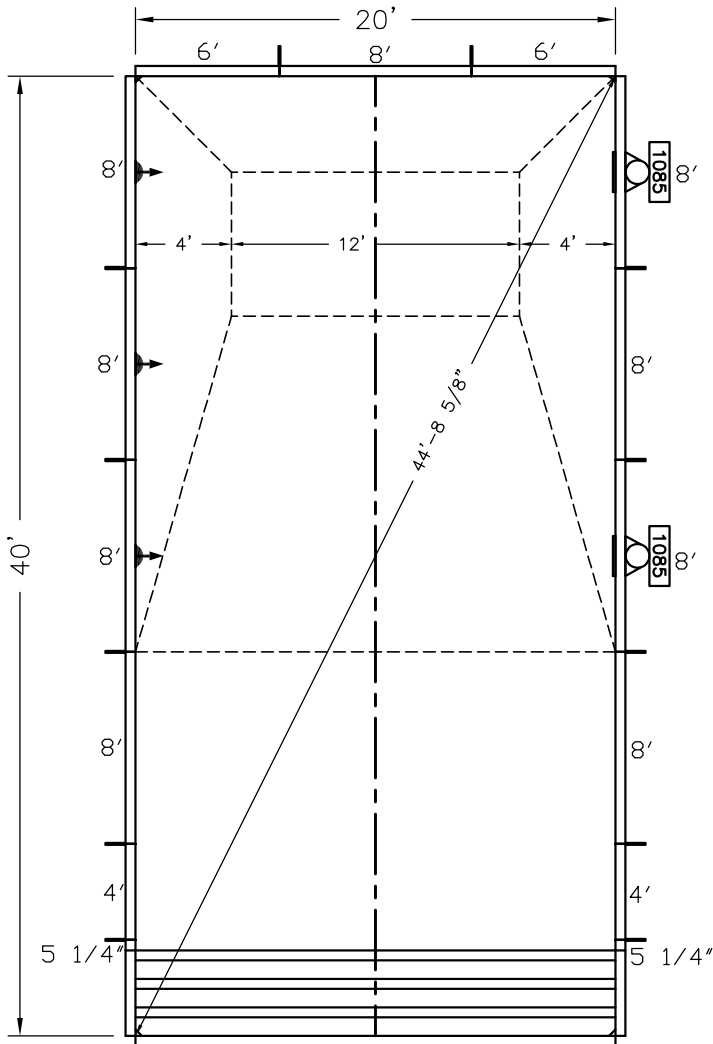
20' POURED STEP W/LINER TRACK SCREED EDGE S2000SP34200XXU
