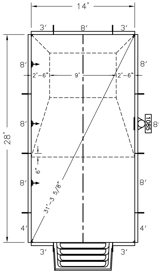
8' PLASTIC STEP
