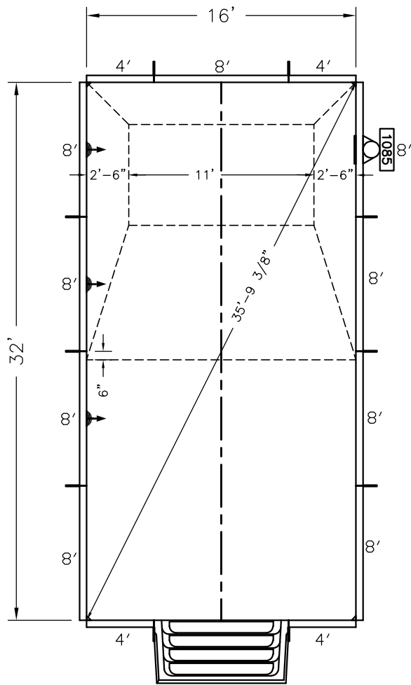
8' PLASTIC STRAIGHT
