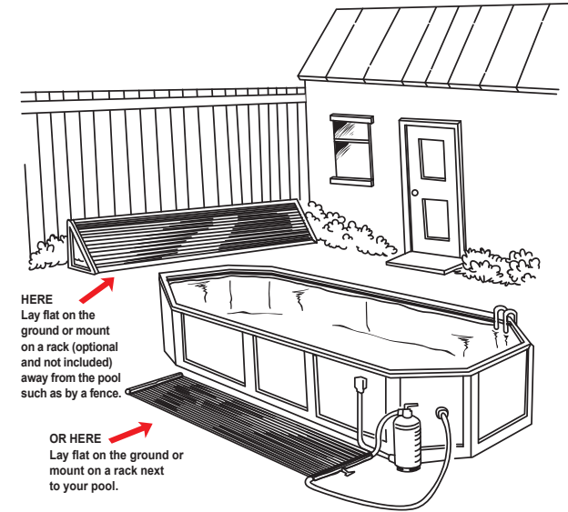
Durable 20 ft. x 4 ft. SunSaver™ solar panel, pre-plumbed
