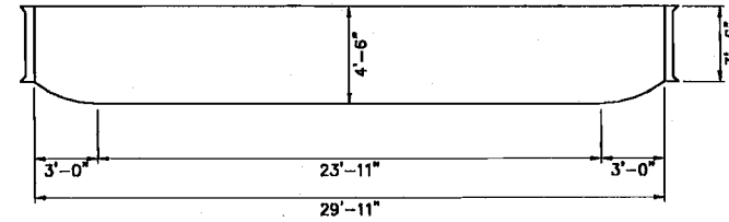
FULL 5' EXPANDABLE BOTTOM VOLUME: 9738 IMP GAL
